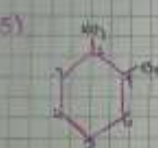
1,2-dibromobenceno o-bromobenceno
