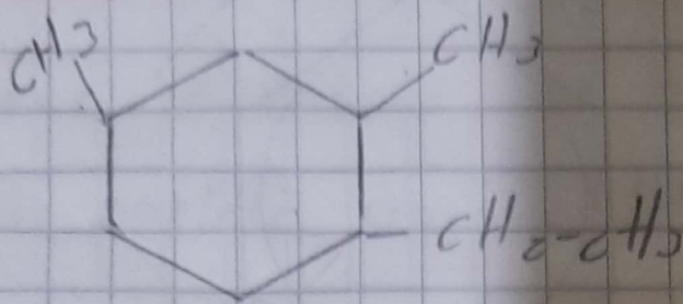
4-ethyl-1,3-dimetilbenceno
