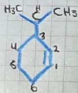
3 isopropilciclohexeno
